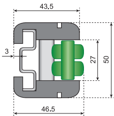
钢侧板 Steel Profile
