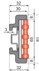
钢侧板 Steel Profile
