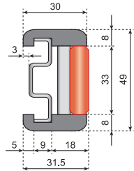
钢侧板 Steel Profile
