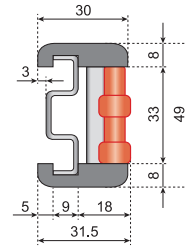
钢侧板 Steel Profile
